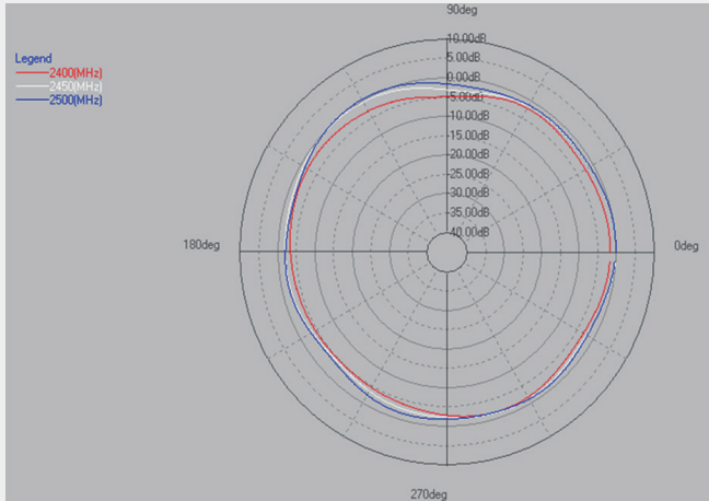
2.4G (PHI=0)
