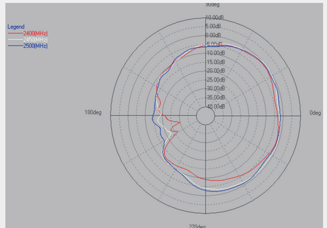
2.4G (PHI=90)
